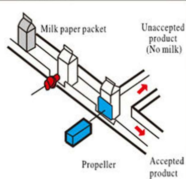
Capacitive type proximity switch
