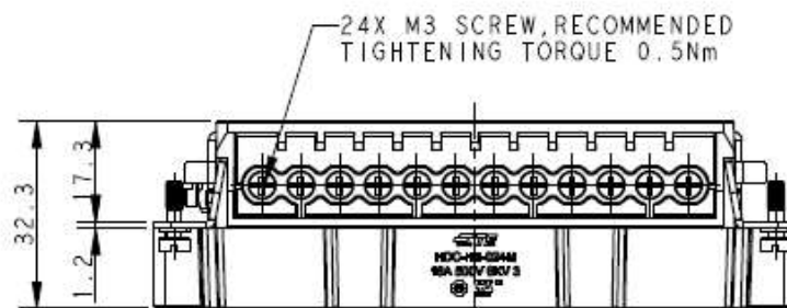
TYPE 1, T2040242101-000, WITH LOGO
