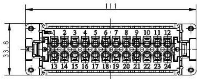
24X M3 SCREW, RECOMMENDED TIGHTENING TORQUE 0.5Nm
