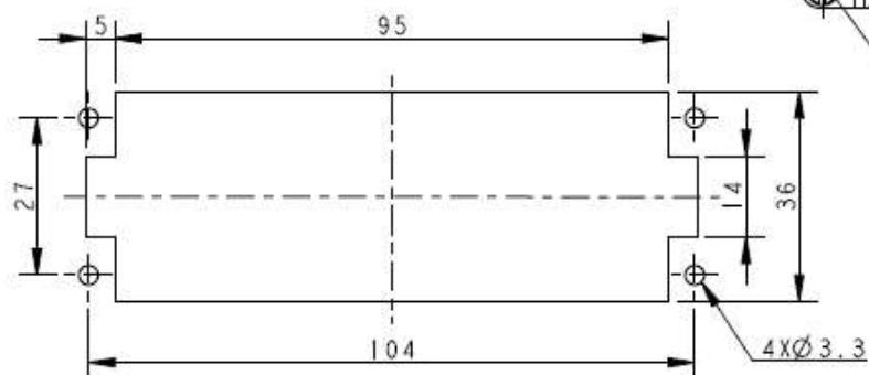
PANEL CUT FOR INSERTS FOR USE WITHOUT HOODS/ HOUSINGS
