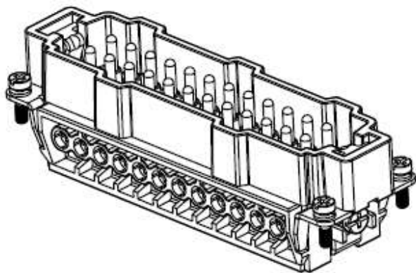
TYPE 2, T2040242101-001, WITHOUT LOGO
