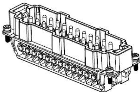
TYPE 1, T2040242101-000, WITH LOGO
