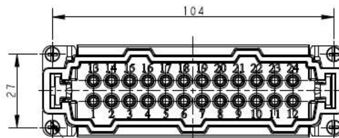
4X M3 SCREW, RECOMMENDED TIGHTENING TORQUE 0.5Nm
