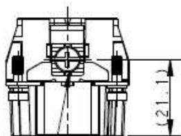
TYPE 1, T2040242101-000, WITH LOGO
